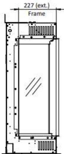
Left view
