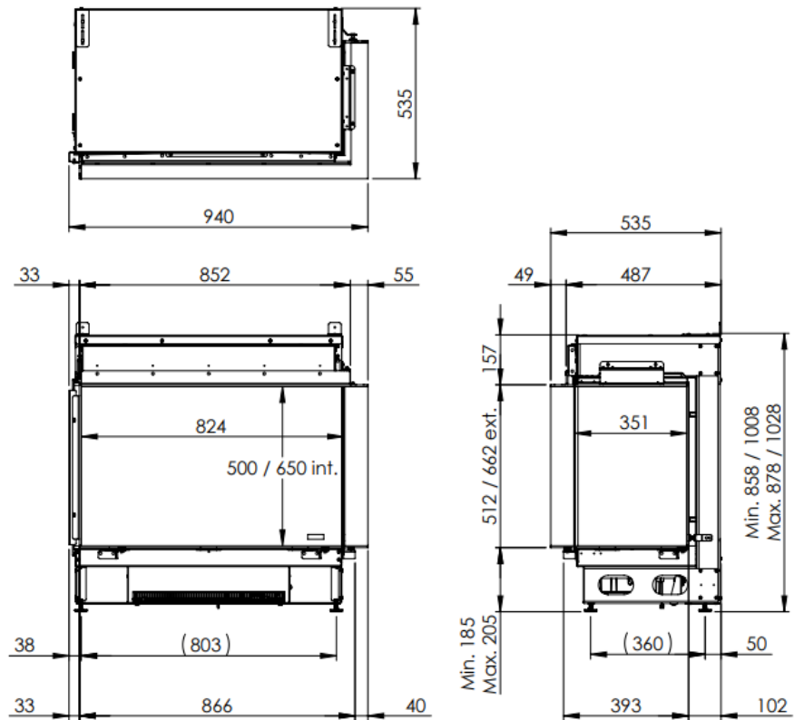
Dimensional Drawing e-Matrix 800x500-650 IIR (MkII)
